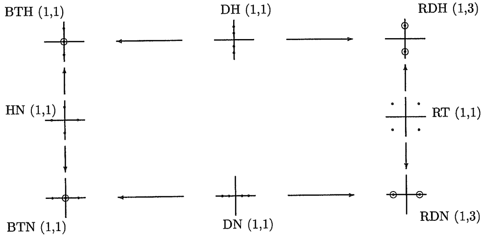
Figure 1: 8 types of matrices A where 2A \odot I_n has rank defect 2
